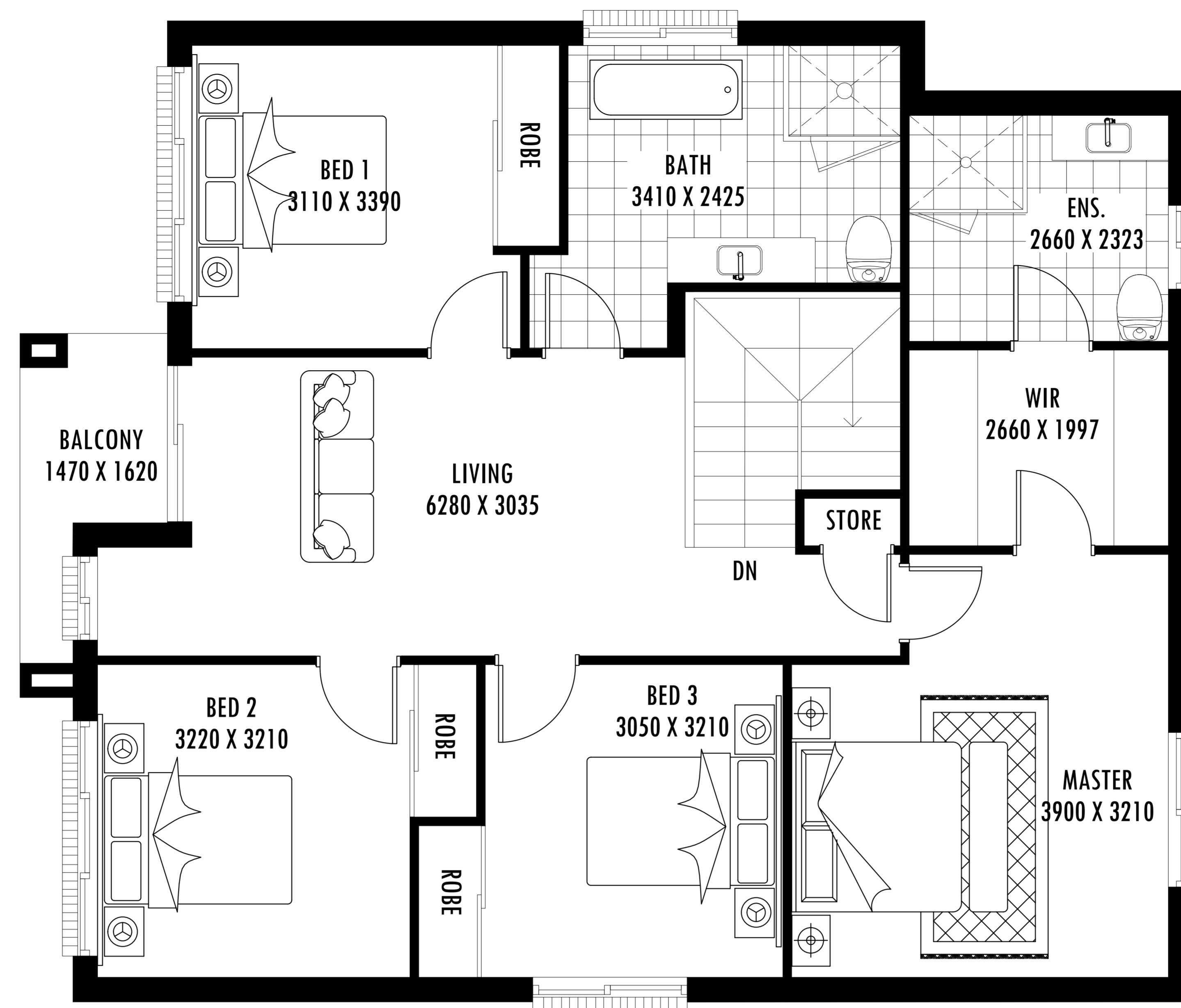
UPPER FLOOR
