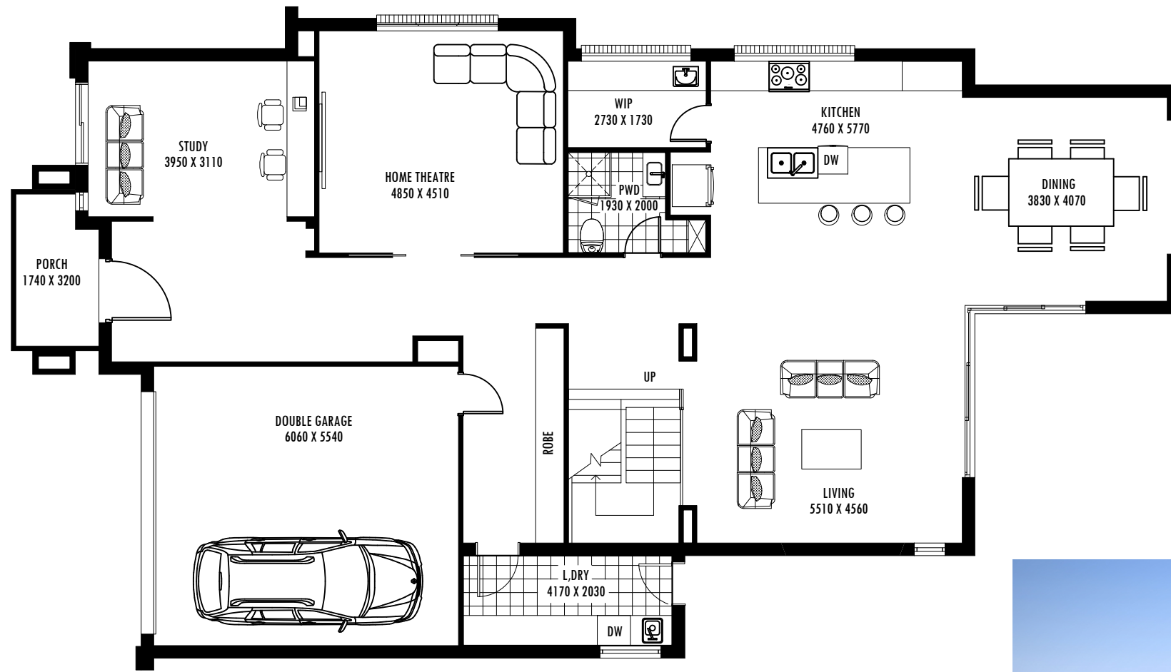
GROUND FLOOR
